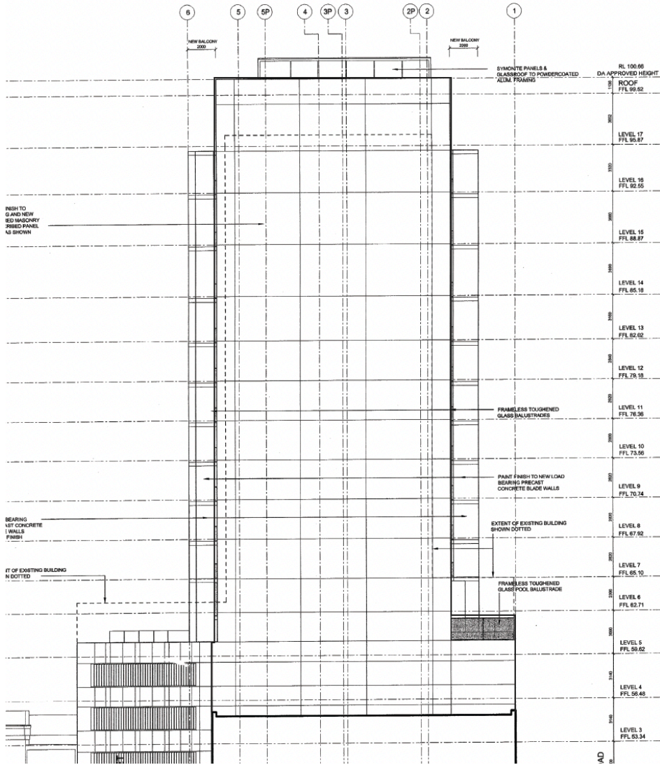
Figure 2. Western Elevation
